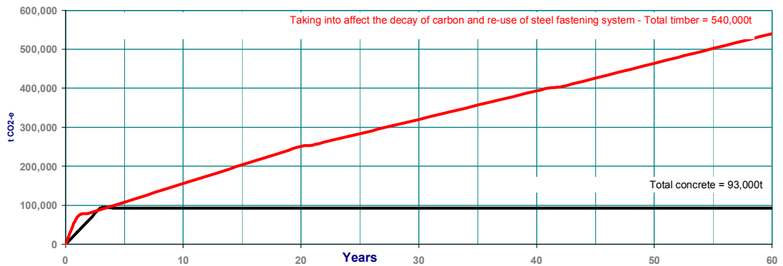
Figure 3. Concrete versus Timber with re-used fittings plus emissions from timber decay
